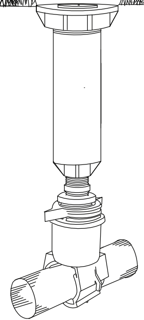
BS 2575 with 3/4" to 1/2" Riser Application
